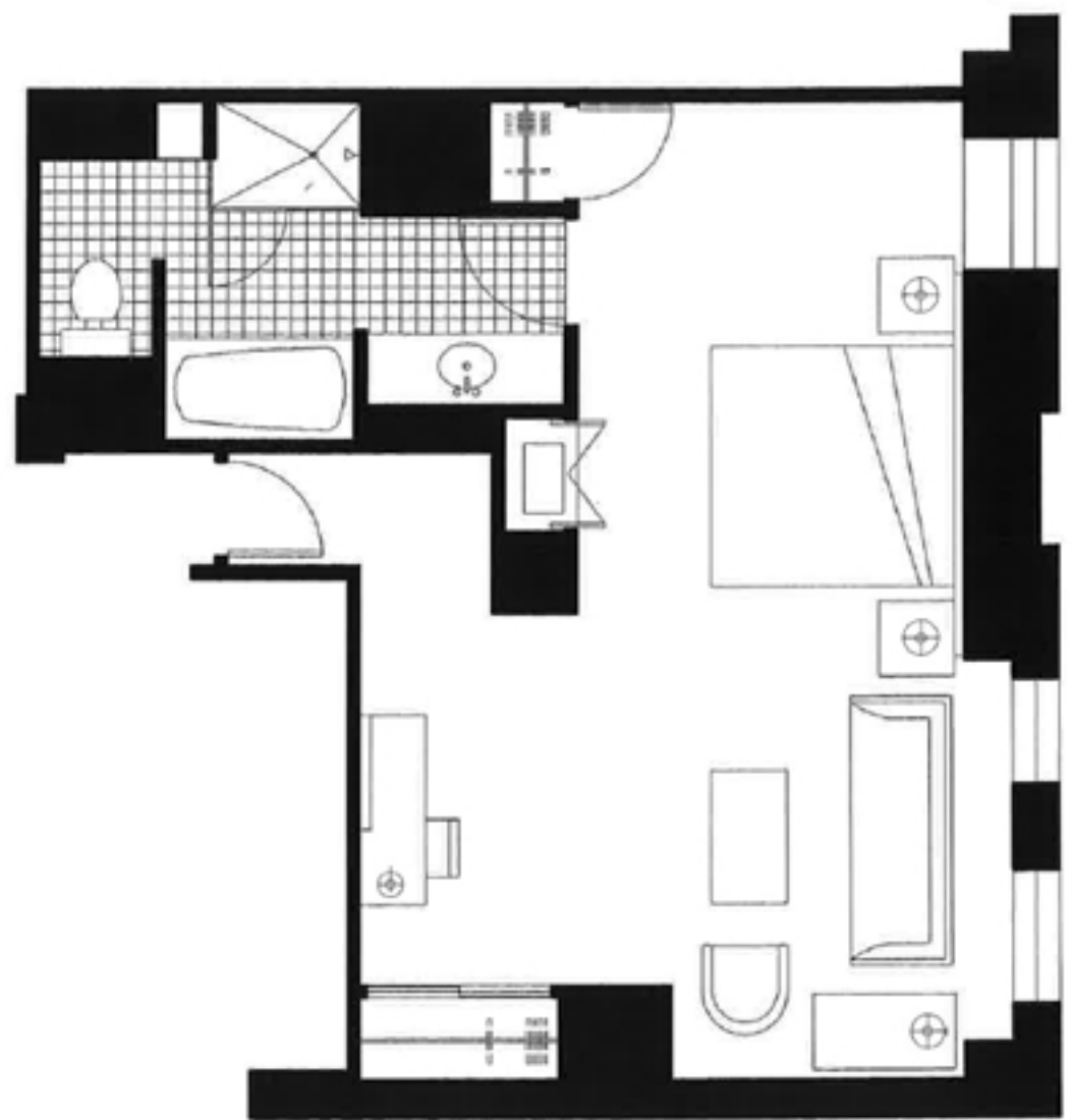
ROOM 01, 02 (7 KING BED) FLOOR PLAN 3/16"=1'-0"
