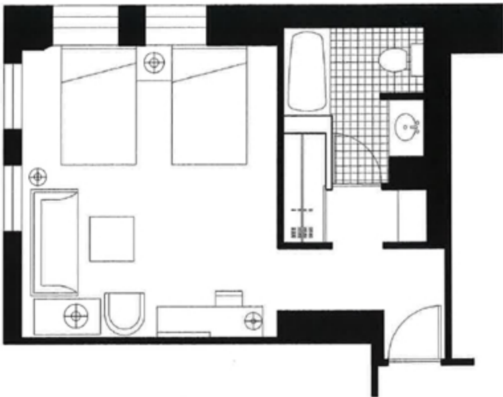
ROOM 08 (10 DOUBLE DOUBLE) FLOOR PLAN 3/16"=1'-0"
