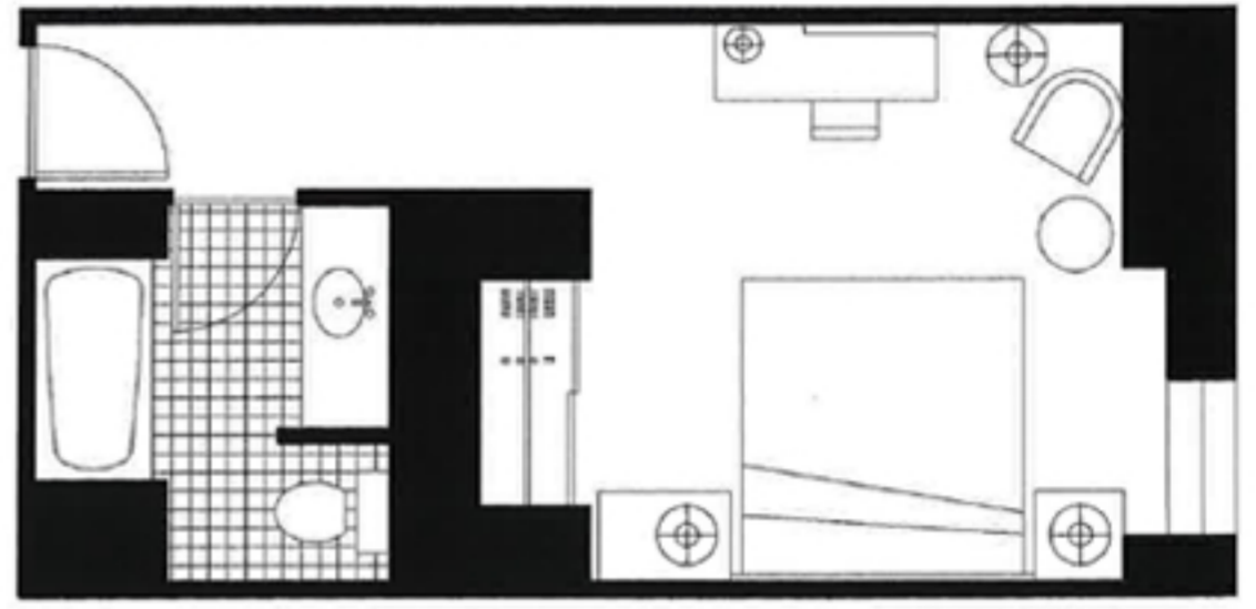
ROOM 03 (13 KING BED) FLOOR PLAN 3/16"=1'-0"
