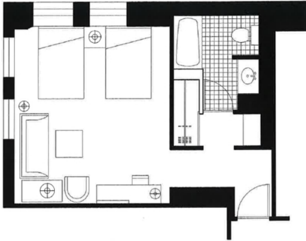
ROOM 08 (10 DOUBLE DOUBLE) FLOOR PLAN 3/16"=1'-0"
